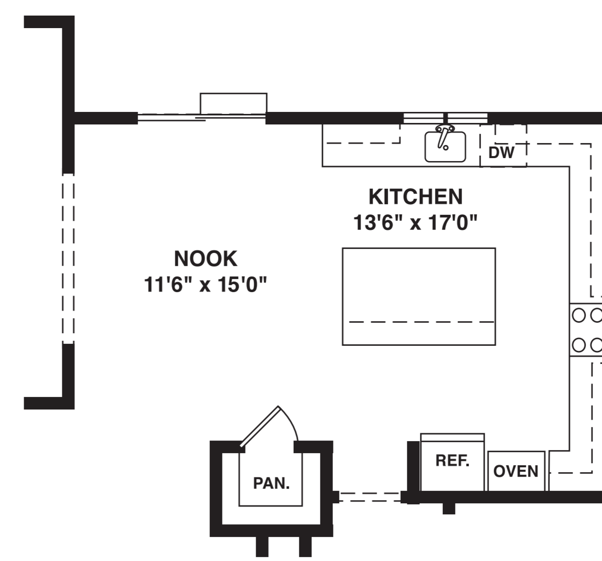
OPT. KITCHEN/NOOK EXTENSION
